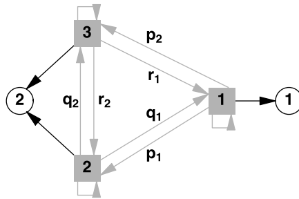
Fig. 1 Schematic representation of the hidden Markov process defined by (66–70). The gray squares and gray arrows indicate, respectively, on the realizations of the internal Markov process and transitions between the realizations; see (69). The circles and black arrows indicate on the realizations of the observed process. The gray arrows are probabilistic; the corresponding probabilities are indicated next to them. The black arrows are deterministic; see (66)
